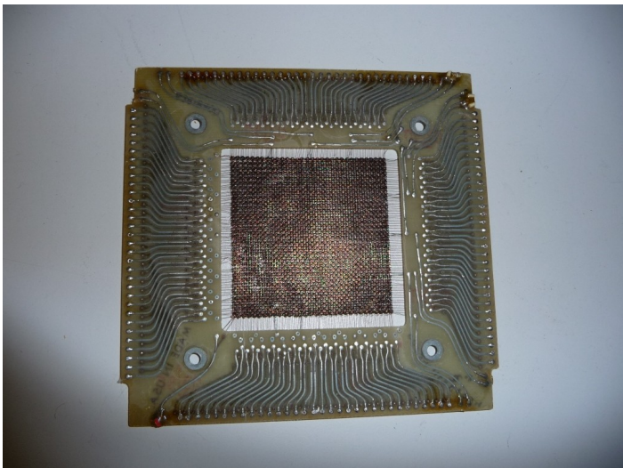
4 kByte Memory
