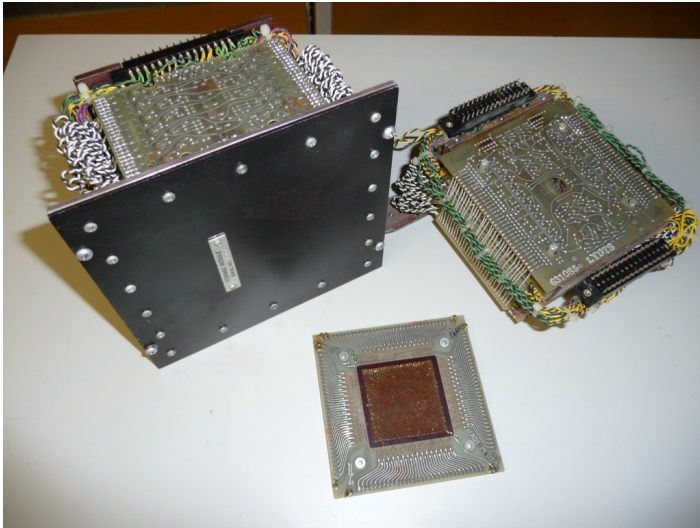
CDC 6500 Memory Stack
