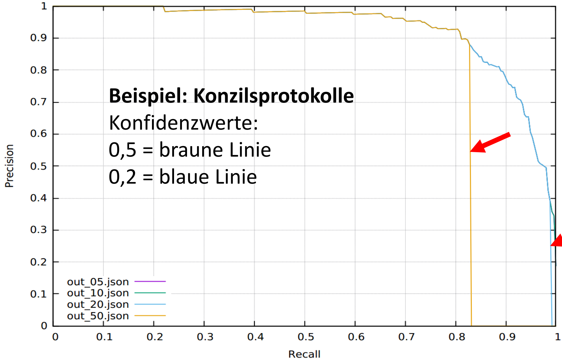
Precision-Recall-Curve
