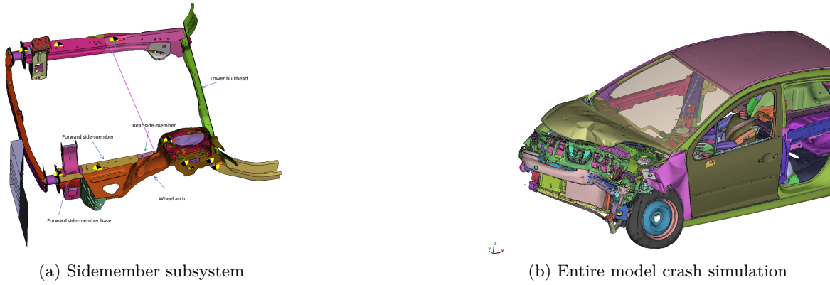
Figure 14: Sidemember subsystem.
