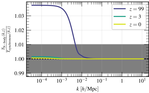
Figure 1. Ratio between the CDM+baryon transfer functions in the N-body gauge (as used for the N-body simulations in this work) and the synchronous gauge at three different redshifts. At redshift z = 99 where the initial conditions are realised, the two gauges lead to transfer functions differing by almost 4% at very large scales. At the k \sim 0.006 h \text{ Mpc}^{-1} corresponding to the fundamental k -mode of the simulations that will be used to construct EuclidEmulator2 (see section 4), the effect is just about at the 1% level.
