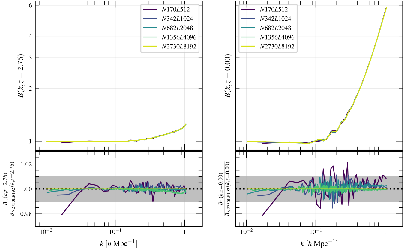
Figure 2. Convergence test results for volume of the NLC factor B(k,z) of simulations with L \in \{512, 1024, 2048, 4096, 8192\} h^{-1} Mpc. We show results for two different redshifts. Apart from individual k modes on mildly nonlinear scales, simulation boxes with L = 1024 h^{-1} Mpc are converged at the 1% level.
