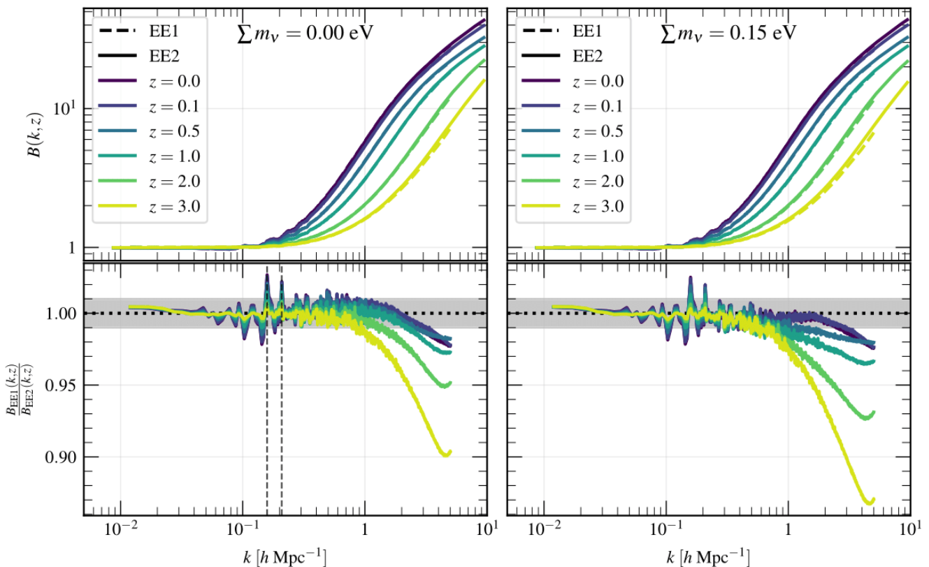
Figure 11. In this figure we compare the NLC prediction of EuclidEmulator2 to that of EuclidEmulator1 for two cosmologies: one for which \sum m_\nu = 0.00 eV (left panel) and \sum m_\nu = 0.15 eV for the other (right panel). A_s is the same in both cosmologies, however the value of \sigma_8 differs due to the mass difference in the neutrino sector. It is not surprising that the agreement on the largest scales is nearly perfect for both cosmologies as both emulators return values close to unity irrespective of the cosmology by construction. The oscillations around BAO scales are due to cosmic variance. The vertical, black, dashed lines indicate the two k -modes where the curves for EuclidEmulator1 and EuclidEmulator2 deviate the most from each other in Fig. 12. The time-dependent mismatch on small scales is due to the different mass resolutions of the training of the two emulators. A key point is that this plot shows that the agreement between EuclidEmulator1 and EuclidEmulator2 is not only very good for massless neutrino cosmologies where EuclidEmulator1 is supposed to work well by construction, but also for w_0 CDM+ \sum m_\nu models which EuclidEmulator1 was not designed for. This suggests that EuclidEmulator1 is able to predict the nonlinear power spectrum within 1% of accuracy for z < 0.5 even if the cosmology contains massive neutrinos (of course, the linear power spectrum must be computed taking the neutrino masses into account).
