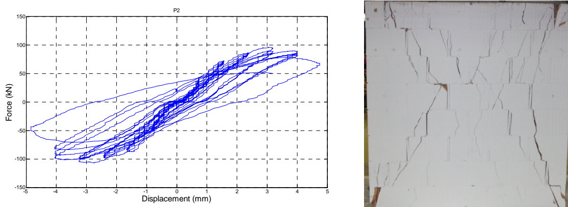
Figure 5: Hysteretic Response of Wall P2
