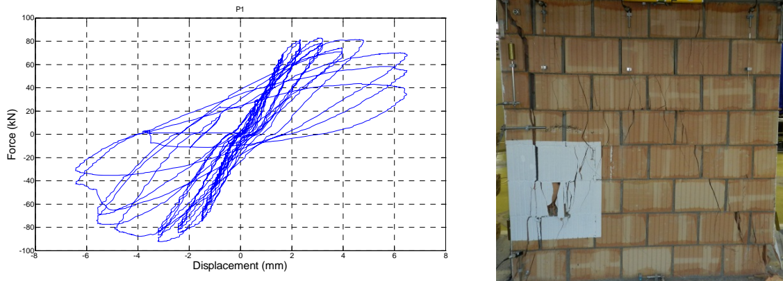
Figure 4: Hysteretic Response of Wall P1
