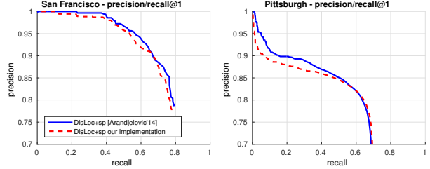
Figure 2. Precision-recall curves obtained by a state-of-the-art localization recognition system [2] when considering the top-ranked image after spatial verification (raw inlier count re-ranking).
