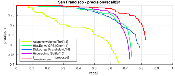
Figure 7. Combining [2] with our proposed scheme for handling geometric bursts not only provides significantly better results over the original method but also outperforms state-of-the-art methods for both place recognition and image-based localization.
