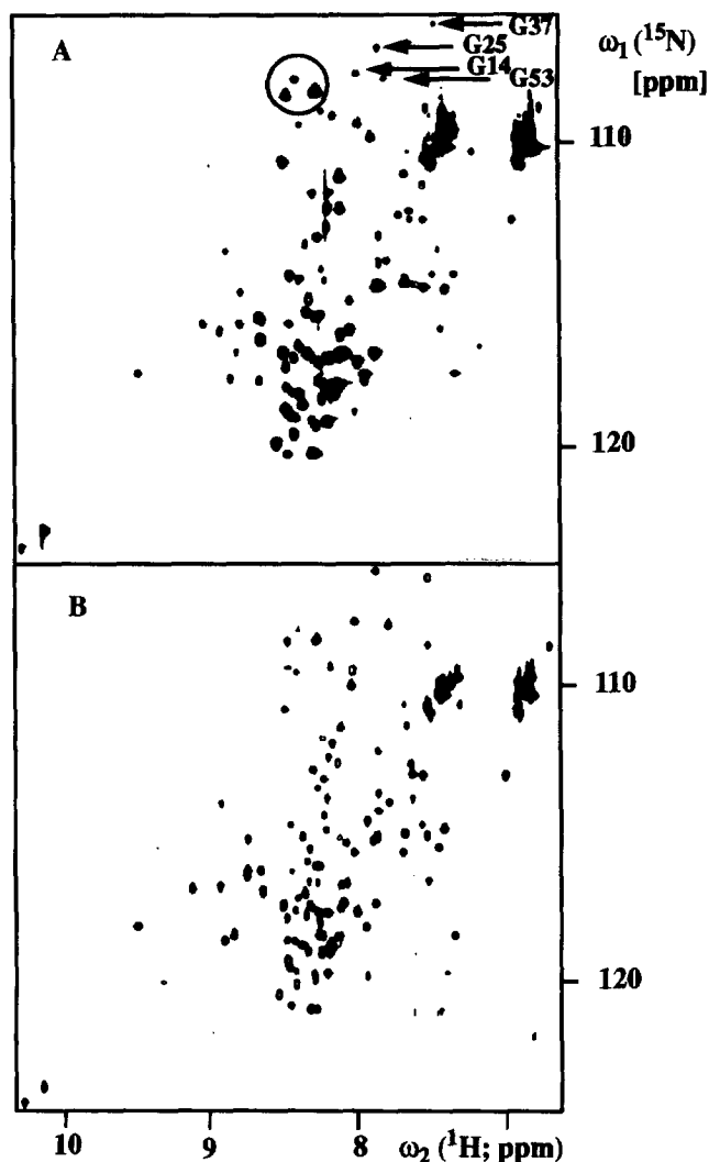
Fig. 1. [ ^{15}\text{N} , ^1\text{H} ]-COSY spectra of 434-repressor(1–63) (protein concentration 4 mM, solvent 90% \text{H}_2\text{O} /10% \text{D}_2\text{O} , urea concentration 7 M, pH 7.6, temperature 291 K, ^1\text{H} frequency 500 MHz). (A) Without addition of salt. Arrows indicate the positions of four glyceryl resonances in the folded protein, the circle encloses the corresponding peaks of the unfolded conformation [17]. (B) After addition of 0.2 M sodium trifluoroacetate.
