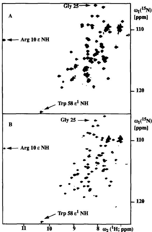
Fig. 3. [ ^{15}\text{N} , ^1\text{H} ]-COSY spectra of 434-repressor(1–63) in 6 M urea after addition of salts. (protein concentration 4 mM, solvent 90% \text{H}_2\text{O}/10\% \text{D}_2\text{O} , pH 7.6, temperature 291 K, ^1\text{H} -frequency 500 MHz). (A) 0.5 M sodium trifluoroacetate; (B) 1.8 M sodium chloride. The resonances of Arg-10 \epsilon\text{NH} , Gly-25 and Trp-58 \epsilon^1\text{NH} are identified by arrows.
