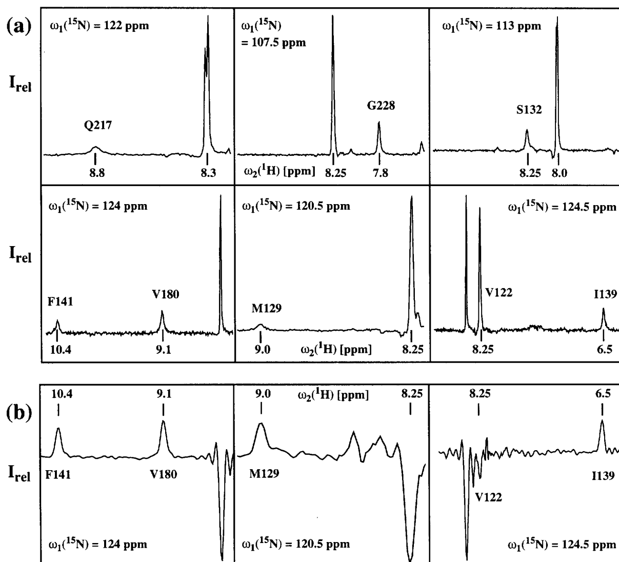
Fig. 5. (a) Cross sections along the \omega_2(^1\text{H}) frequency taken at the positions indicated with horizontal bars in the ^{15}\text{N},^1\text{H} -COSY spectrum of Fig. 4a. To allow for the fact that the \omega_1(^{15}\text{N}) positions of the individual peaks contained in a given cross section may be slightly different, cross sections taken exactly on-resonance for each individual peak in the cross section were added to obtain the correct representation of the relative peak intensities. (b) Cross sections through the ^{15}\text{N}\{^1\text{H}\} -COSY-related ^{15}\text{N}\{^1\text{H}\} -NOE spectrum of Fig. 4, c+d. The resonances belonging to residues in the assigned segment 121–231 of mPrP (23–231) are identified by residue type and sequence position.
