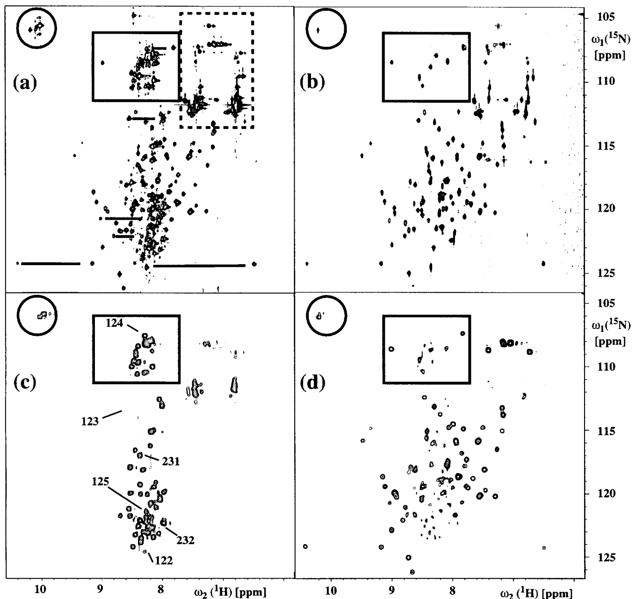
Fig. 4. (a) ^{15}\text{N}, ^1\text{H} -COSY spectrum of mPrP (23–231). The horizontal bars indicate the locations of the cross sections shown in Fig. 5a. The rectangle drawn with broken lines surrounds the spectral region of the side chain amide and guanidino resonances. (b) ^{15}\text{N}, ^1\text{H} -COSY spectrum of mPrP (121–231). (c) Subspectrum containing the negative peaks from a ^{15}\text{N}[^1\text{H}] -COSY-relayed ^{15}\text{N}\{^1\text{H}\} -NOE experiment with mPrP (23–231). The peaks that were individually assigned to residues in the polypeptide segment 121–231 are identified with the residue number. (d) Subspectrum containing the positive peaks from the same experiment as (c). In all four spectra the circle contains the Trp indole ^{15}\text{N}^{\epsilon}\text{-}^1\text{H} cross peaks, and the rectangle the Gly backbone ^{15}\text{N}\text{-}^1\text{H}^{\text{N}} peaks.
