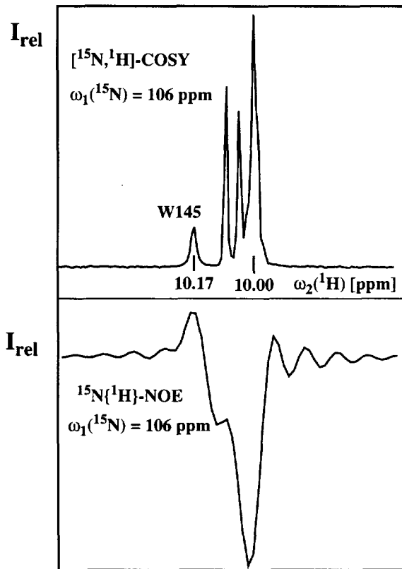
Fig. 6. Cross sections through the spectra (a) and (c+d) in Fig. 4, showing the resonances of the indole ^{15}\text{N}^{\epsilon}\text{-}^1\text{H} moieties of the eight tryptophan residues in mPrP (23-231). The cross sections were obtained as described in the caption to Fig. 5. The peak of the single Trp residue from the assigned polypeptide segment 121-231 is identified in the top trace.
