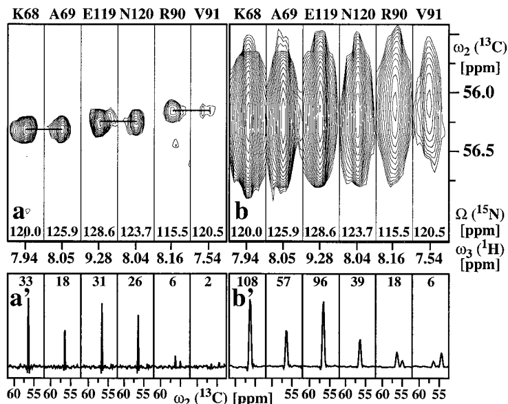
Figure 2. Comparison of corresponding [\omega_2(^{13}\text{C}), \omega_3(^1\text{H})] strips from HNCA spectra obtained with and without ^{13}\text{C} constant time evolution: (a) [^{13}\text{C}] -ct- [^{15}\text{N}, ^1\text{H}] -TROSY-HNCA recorded with the scheme of Figure 1; (b) [^{15}\text{N}, ^1\text{H}] -TROSY-HNCA (Salzmann et al., 1998). The strips were taken at the ^{15}\text{N} chemical shifts indicated at the bottom, and are centered about the corresponding ^1\text{H}^N chemical shifts. At the top the sequence-specific assignments are indicated by the one-letter amino acid symbol and the sequence number. In (a) the three sequential connectivities are indicated by horizontal lines. (a') and (b') show cross sections along the \omega_2(^{13}\text{C}) dimension through the centers of the strips in (a) and (b), respectively, where the chemical shift range from 52 to 62 ppm is plotted. The signal-to-noise ratios for the main peak in each cross section are indicated at the top. Both spectra were recorded at 20 °C with the same 0.5 mM sample of uniformly ^2\text{H}/^{13}\text{C}/^{15}\text{N} -labeled 7,8-dihydroneopterin aldolase from S. aureus (Hennig et al., 1998) in a mixed solvent of 95% \text{H}_2\text{O}/5\% \text{D}_2\text{O} at pH 6.5, using a Bruker DRX-750 spectrometer equipped with four rf channels for generating the ^1\text{H} , ^2\text{H} , ^{13}\text{C} and ^{15}\text{N} rf-pulses, a pulsed field gradient unit and a triple resonance probehead with an actively shielded z-gradient coil. When recording the spectrum (b), the previous implementation of the [^{15}\text{N}, ^1\text{H}] -TROSY-HNCA experiment (Salzmann et al., 1998) was modified so that ^{13}\text{CO} decoupling by Gaussian off-resonance pulses was replaced by 0.83 kHz off-resonance SEDUCE-1 decoupling (McCoy and Mueller, 1992) and the rf-pulses on the ^{13}\text{C}^\alpha channel were applied with a field strength of 20.83 kHz, exactly as described for [^{13}\text{C}] -ct- [^{15}\text{N}, ^1\text{H}] -TROSY-HNCA in Figure 1. The following parameter settings were used for (a): data size 42(t_1) \times 128(t_2) \times 1024(t_3) complex points; t_{1\text{max}}(^{15}\text{N}) = 17.4 , t_{2\text{max}}(^{13}\text{C}^\alpha) = 25.6 , t_{3\text{max}}(^1\text{H}) = 75.6 ms; spectral widths in \omega_1(^{15}\text{N}) , \omega_2(^{13}\text{C}^\alpha) and \omega_3(^1\text{H}) 2400, 5000 and 13550 Hz, respectively; 16 scans per increment were acquired, resulting in 4 days of measuring time. The data set was zero-filled to 128(t_1) \times 256(t_2) \times 2048(t_3) complex points. In (b) the same parameters were used except for the following: data size in t_2 was 40 points, t_{2\text{max}}(^{13}\text{C}^\alpha) = 8 ms, 48 scans per increment were acquired in 4 days of measuring time, and zero-filling in t_2 was to 128 complex points. Prior to Fourier transformation both data matrices were multiplied with a 75^\circ -shifted sine bell window in the indirect dimensions and a 60^\circ -shifted sine bell window in the acquisition dimension (DeMarco and Wüthrich, 1976). Data processing was performed using the program PROSA (Güntert et al., 1992), and for the data analysis the program XEASY (Bartels et al., 1995) was used.
