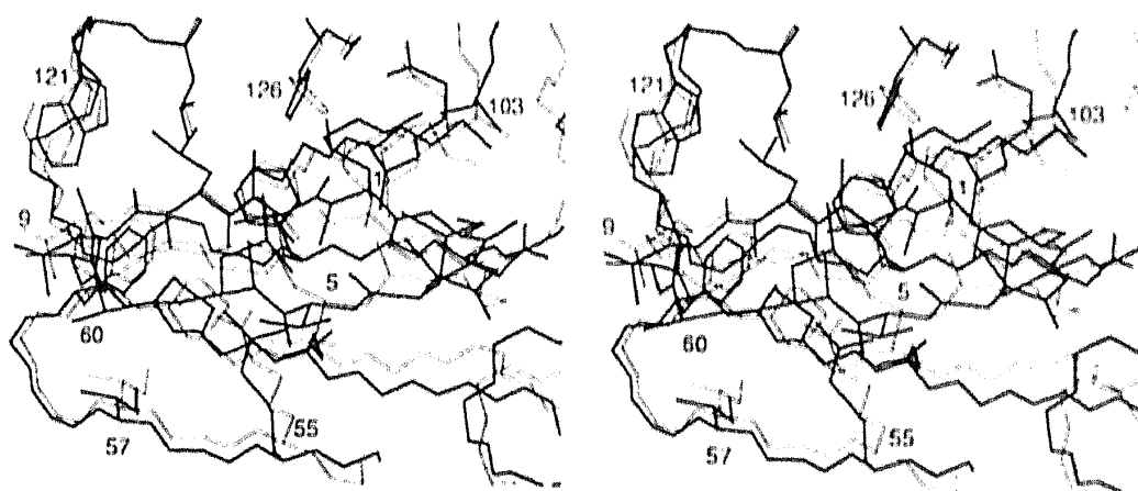
Fig. 8. Stereoview of the binding site in the NMR conformer with the lowest residual energy of the Cyp-CsA complex (thick line) and comparison to the crystal structure of Pflügl et al. (1993) (thin line). The backbone atoms N, C \alpha and C \beta of the binding-area residues as defined in footnote d of Table 2 have been superimposed for minimal rmsd. For the NMR conformer, all side chains of CsA and those of Cyp that belong to the ligand binding site are shown. For improved clarity, the solvent-exposed side chains of CsA have been omitted from the crystal structure.
