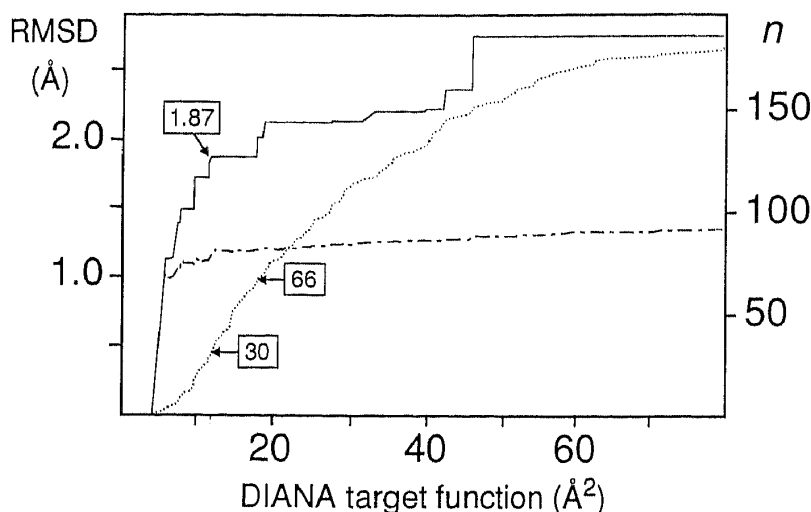
Fig. 4. Selection of a group of 'best' DIANA conformers of the Cyp–CsA complex. Of the 200 conformers, 180 ( n on the right) had residual target function values \leq 80 Å 2 (plotted along the horizontal axis). The conformers were arranged according to the residual DIANA target function value, and the dotted line represents the number of conformers with target functions below the value on the horizontal axis. For each conformer the maximal pairwise rmsd, \text{rmsd}_{\text{max}} , relative to all conformers with smaller target functions is plotted (solid line), and the dash-dotted line represents the average of all these pairwise rmsd values. Rmsd values were calculated for the backbone atoms N, C α and C β of residues 3–39, 53–63, 91–102, 111–118, 129–143 and 154–164 of Cyp and all residues of CsA, which were found to be well defined after a preliminary analysis of the DIANA conformers.
