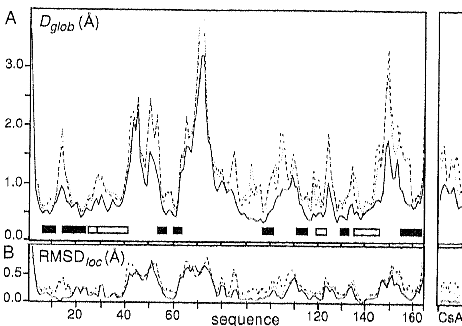
Fig. 5. Comparison of the local backbone conformations of the NMR solution structure, the X-ray crystal structure (Pflügl et al., 1993) and the previously reported molecular model (Spitzfaden et al., 1992a) of the Cyp-CsA complex. (A) Plots against the amino acid sequence of the average global backbone displacement ( D_{glob} ) (Billeter et al., 1989) relative to the mean NMR structure (solid line) for the individual amino acid residues of the 22 energy-minimized conformers after superposition of the backbone atoms N, C ^{\alpha} and C ^{\beta} in the well-ordered segments 3-65 and 76-164 of Cyp and all residues of CsA. The rmsd values relative to the crystal structure (dotted line), and relative to the molecular model of Spitzfaden et al. (1992a) (dashed line) are also given. (B) Local backbone rmsd relative to the mean NMR coordinates (solid line) ( rmsd_{loc} ), calculated for all continuous tripeptide segments along the sequence and plotted for the central residues. The rmsd values relative to the crystal structure (dotted line) and the model (dashed line) are also shown. Horizontal bars indicate regions of regular secondary structure: black bars, \beta -sheets; open bars, \alpha - or 3_{10} -helices.
