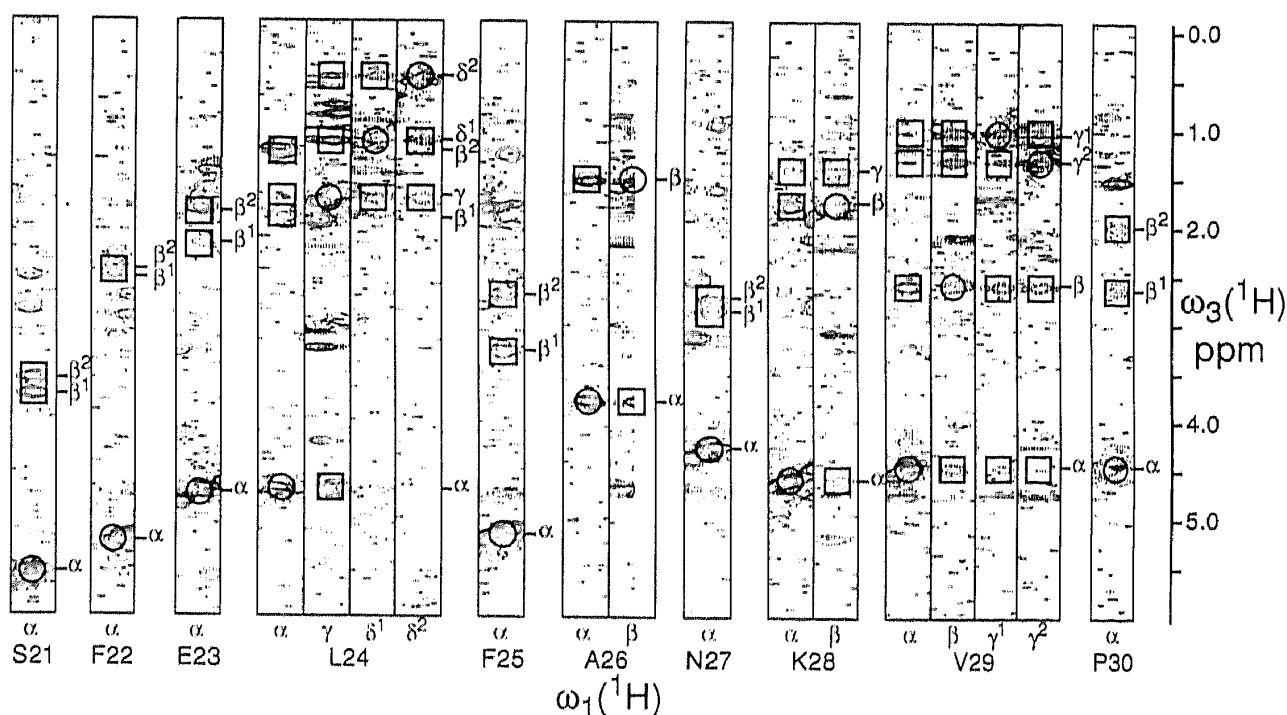
Fig. 1. Illustration of the amino acid side-chain resonance assignments for the segment Ser 21 –Pro 30 of the Cyp polypeptide chain. For each residue, selected regions (strips) from \omega_1(^1\text{H}) – \omega_3(^1\text{H}) -planes of a 3D ct-[HCCH]-TOCSY spectrum, recorded with a mixing time of 7 ms (see Table 1), of a complex between uniformly [ ^{13}\text{C}, ^{15}\text{N} ]-doubly labeled Cyp and unlabeled CsA are shown. Strips along \omega_3(^1\text{H}) with a width of 0.2 ppm in the \omega_1(^1\text{H}) -dimension were taken at the ^{13}\text{C} frequencies of the ( ^1\text{H}, ^{13}\text{C} )-direct correlation peaks ( \omega_1 = \omega_3 , indicated by circles). The individual strips are identified by the atom positions on the right, and the spin-system assignments at the bottom (the strip for Ala 26 \beta was at the edge of the spectral width along \omega_1 , and therefore the right half of the signal is truncated). TOCSY cross peaks along the \omega_3 dimension are indicated by boxes and assignments are given on the right side of the presentation for each residue. Dashed lines indicate negative signal intensities of folded peaks.
