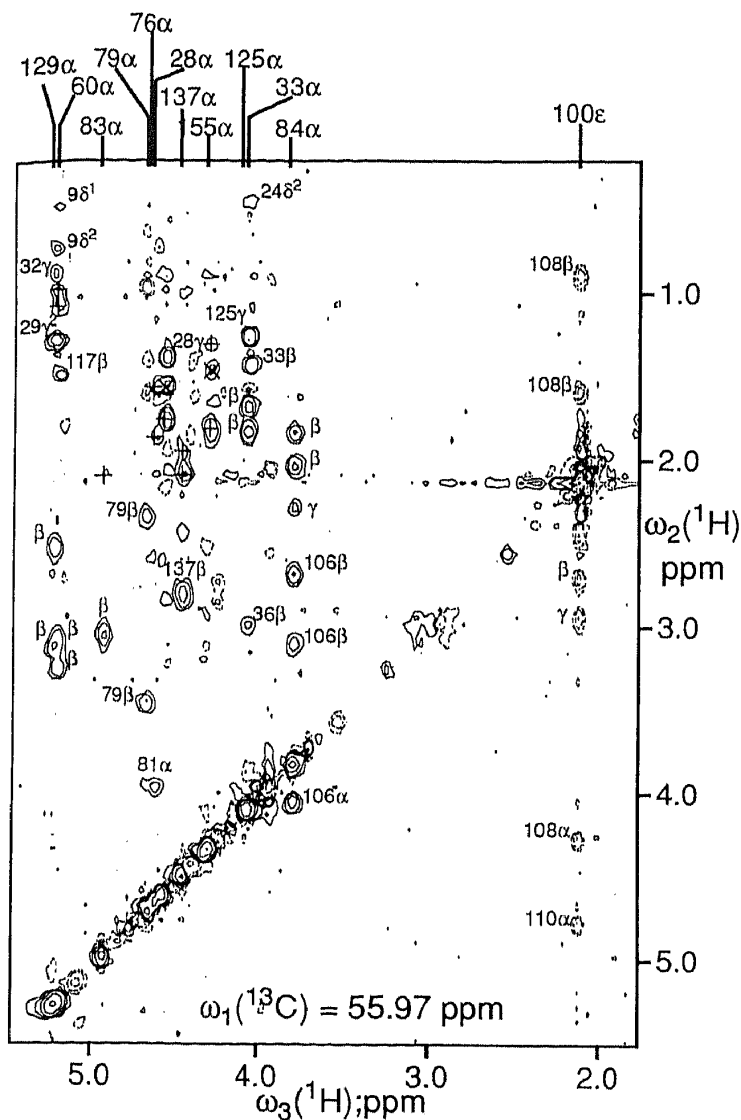
Fig. 2. Region ( \omega_2(^1\text{H}) = 0.2\text{--}5.3 ppm, \omega_3(^1\text{H}) = 1.8\text{--}5.3 ppm) of the [ ^1\text{H}, ^1\text{H} ]-plane at \omega_1(^{13}\text{C}) = 55.97 ppm from a 3D ^{13}\text{C} -correlated [ ^1\text{H}, ^1\text{H} ]-NOESY spectrum of a complex between uniformly [ ^{13}\text{C}, ^{15}\text{N} ]-doubly labeled Cyp and unlabeled CsA. The selected area contains all the signals in this particular [ ^1\text{H}, ^1\text{H} ]-plane. The assignments of the direct 'diagonal' correlation peaks ( \omega_2 = \omega_3 ) present in this plane are given at the top of the spectrum by the residue number and the atom position. Some cross peaks are labeled in the spectrum; for intramolecular cross peaks only the atom positions are given, for intermolecular cross peaks also the residue number. In cases of degenerate \text{C}^\alpha\text{H} frequencies along \omega_2 , the labels are positioned on the same side of the cross peaks as the assignment at the top. In crowded regions, + and x indicate assigned and unassigned cross peaks, respectively. Dashed contour lines indicate negative intensity levels of folded peaks.
