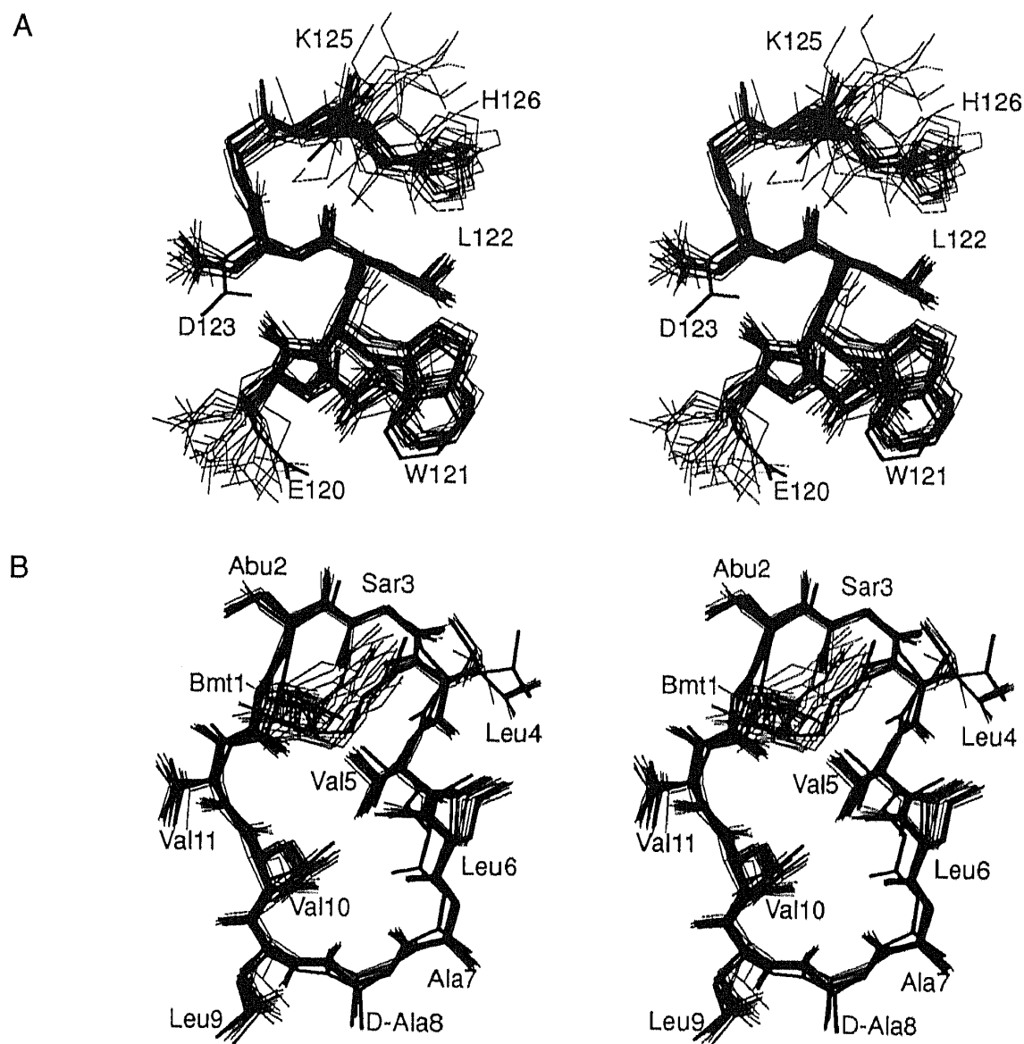
Fig. 7. Local superpositions of the 22 energy-minimized conformers of the solution structure (thin lines) of the Cyp-CsA complex with the crystal structure (thick line) for the following peptide segments: (A) Thr 119 -His 126 (TEWLDGKH); (B) CsA. The backbone atoms N, C α and C' of the individual energy-refined DIANA conformers in the polypeptide segments shown were superimposed for minimal rmsd with the crystal structure of the complex (Pflügl et al., 1993).
