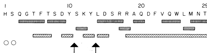
FIG. 6. Amino acid sequence of bovine glucagon and survey of the experimental data by which individual resonance assignments were obtained for the micelle-bound polypeptide. (▬▬▬▬▬▬▬▬) Sequential assignments via d_1 (NOE from \text{NH}_{i+1} to \text{C}^\alpha\text{H}_i ); (▤▤▤▤▤▤▤▤) sequential assignments via d_2 (NOE from \text{NH}_i to \text{NH}_{i+1} ); (▧▧▧▧▧▧▧▧) sequential assignments via d_3 (NOE from \text{NH}_{i+1} to \text{C}^\beta\text{H}_i ); (○) assignment in the sequence relied on the identification of the spin system in the COSY spectrum, whereby the amide proton resonances of these residues were not observed. The arrows indicate locations where all the resonances were assigned but the connectivity between 2 neighbouring residues was not established.
