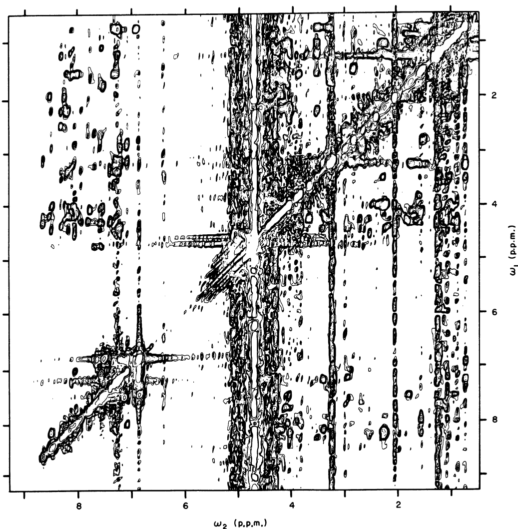
FIG. 7. Contour plot of a 360 MHz 1 H NOESY spectrum observed in the same sample of micelle-bound glucagon as the COSY spectrum of Fig. 5. The spectrum was recorded in 26 h, using a mixing time of 100 ms with random modulation of amplitude 6 ms (Macura et al. , 1981). The digital resolution is 6.3 Hz/point. An absolute value spectrum is shown.
