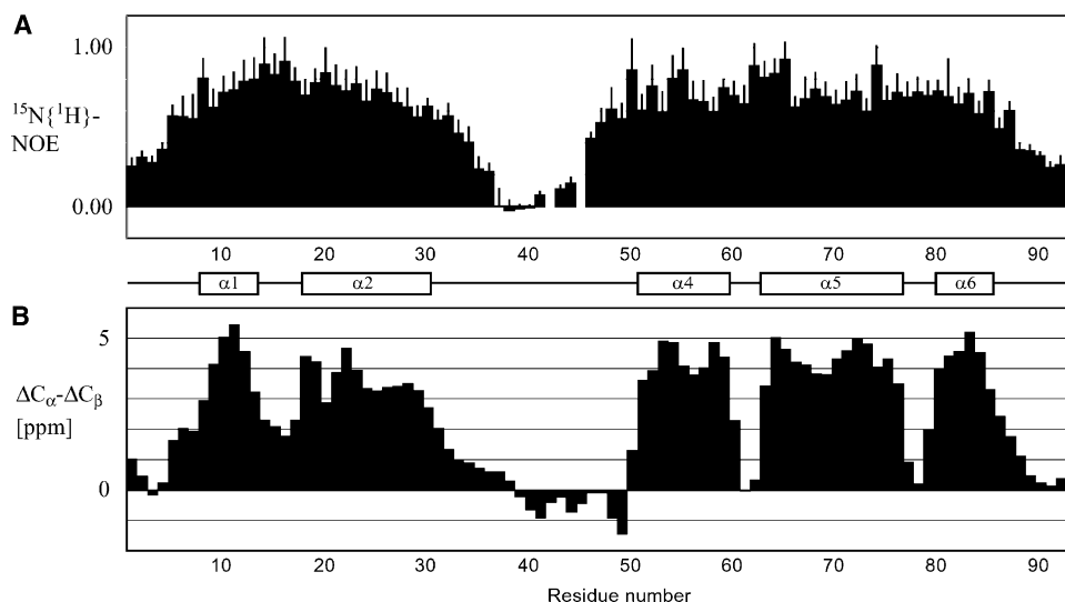
Figure 3. Experiments Showing that NALP1 PYD Is Flexibly Unstructured between Helices α 2 and α 4
