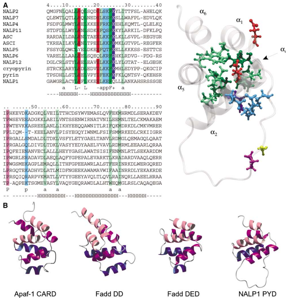
Figure 4. Structural Analysis of the PYD Family
