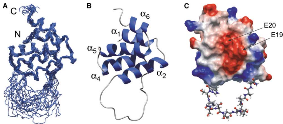
Figure 1. NMR Structure of the NALP1 PYD-Domain: Residues 6–89 Are Shown
