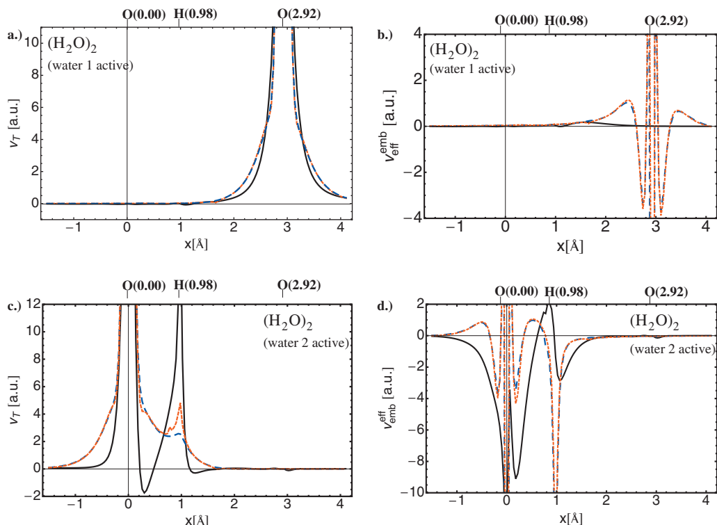
FIG. 6. Comparison of (a) the accurate kinetic-energy component v_T(\mathbf{r}) and (b) the total embedding potentials v_{\text{eff}}^{\text{emb}}(\mathbf{r}) (both black solid line) with approximate potentials obtained using the TF (blue dashed line) and PW91k (red dashed line) functionals for a water dimer with active subsystem 1. [(c) and (d)] Comparison of accurate and approximate potentials for active subsystem 2.
