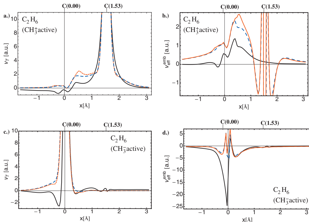
FIG. 9. Comparison of (a) the accurate kinetic-energy component v_T(\mathbf{r}) and (b) the total embedding potentials v_{emb}^{eff}(\mathbf{r}) (both black solid line) with approximate potentials obtained using the TF (blue dashed line) and PW91k (red dashed line) functionals for ethane with CH_3^+ as active subsystem. [(c) and (d)] Comparison of accurate and approximate potentials for ethane with CH_3^- as active subsystem.
