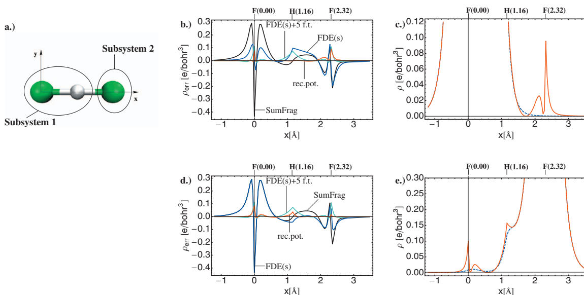
FIG. 2. (a) BP86/QZ4P optimized structure of \text{F-H-F}^- . [(b) and (d)] Difference densities with respect to supermolecular KS-DFT calculation for electron density obtained from the potential reconstruction (rec.pot., red line), the sum of the densities of the isolated fragments (SumFrag, black line), the density from a FDE(s) calculation [FDE(s), blue line], and the density from a FDE(s) employing five freeze-and-thaw cycles [FDE(s)+5 f.t., cyan line] for \text{F-H-F}^- . [(c) and (e)] Comparison of the reference electron density (red solid line) and the one obtained from the potential reconstruction (blue dashed line) for \text{F-H-F}^- . In (b) and (c) subsystem 1 ( \text{F-H} ) is the active subsystem, while in (d) and (e) subsystem 2 ( \text{F}^- ) is active.
