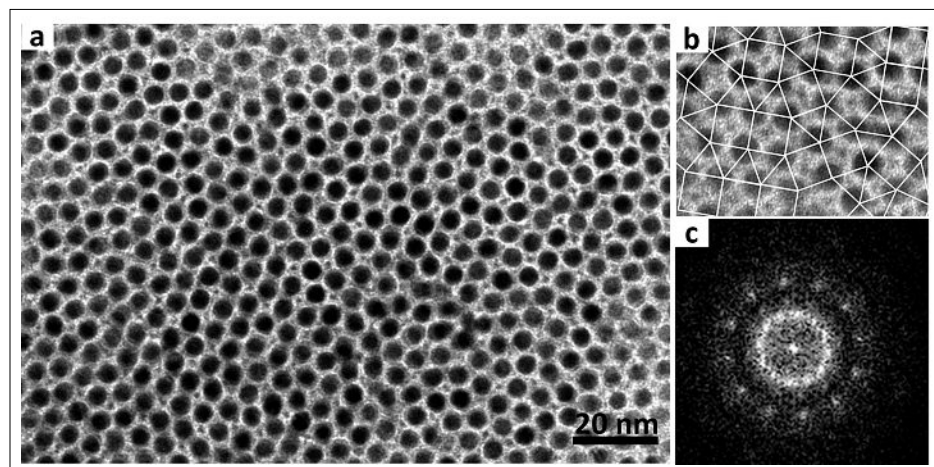
Fig. 7. Dodecagonal quasicrystalline ordering in binary mixtures of 2.9 nm DDA-encapsulated {Mo 132 } clusters and 8.1 nm PbS NCs and ( \gamma_{\text{eff}} = 0.51 ). (a, b) TEM images and (c) FFT pattern from image (a). Reprinted with permission from Nano Lett. 2013, DOI: 10.1021/nl4002475. Copyright 2013 American Chemical Society.
