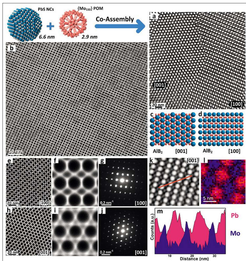
Fig. 6. Detailed structural characterization of AIB 2 -type polyoxometalate/nanocrystal superlattice constructed from dodecylammonium-encapsulated {Mo 132 } clusters and 6.6 nm oleate-capped PbS NCs ( \gamma_{\text{eff}} = 0.58 ). (a, k) HAADF-STEM and (b, e, h) TEM images at various magnifications; (c, d) crystallographic models of [001] and [100] oriented AIB 2 thin-film crystallites; (f, i) images obtained by template analysis of TEM images (e, h); (g, j) small-angle electron diffraction patterns; (l) EDX maps for Pb (red, K-line) and Mo (blue, L-line); (m) EDX line scans for Pb and Mo taken along the line shown in (k). Reprinted with permission from Nano Lett. 2013, DOI: 10.1021/nl4002475. Copyright 2013 American Chemical Society.
