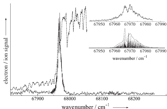
Figure 1. Single-photon photoionization (dashed line) and PFI-ZEKE photoelectron spectrum (full line) of the cyclopentadienyl radical in the region corresponding to the vibrationless \tilde{X}^2E_1'' \rightarrow \tilde{X}^3A_2' transition. The inset shows a comparison of the rotational contour of the origin band (upper trace) with a simulation (lower trace) discussed in the text.
