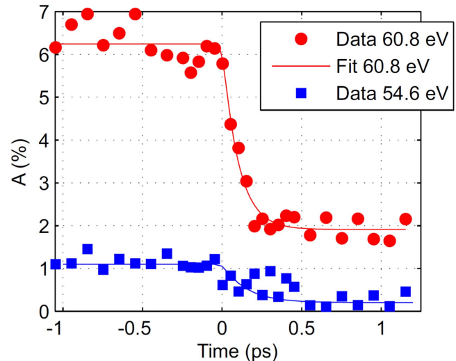
Figure 21. Time-resolved magnetic circular dichroism dynamics around the M_{2,3} edge of Co (60.8 eV). The nonlinear least-square fit reveals a mono-exponential decay with a demagnetization time constant of (92 \pm 22) fs, convoluted with a 59 fs instrument response function. Reprinted figure with permission from [173], Copyright 2015 by the American Physical Society.
