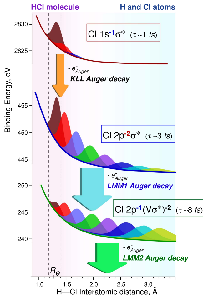
Figure 6. Potential energy curves for different steps of the KLL Auger cascade following Cl 1s \rightarrow \sigma^* excitation. Wave-function distributions are shown in different colors for up to 8 fs after x-ray photon absorption with 1 fs increments.
