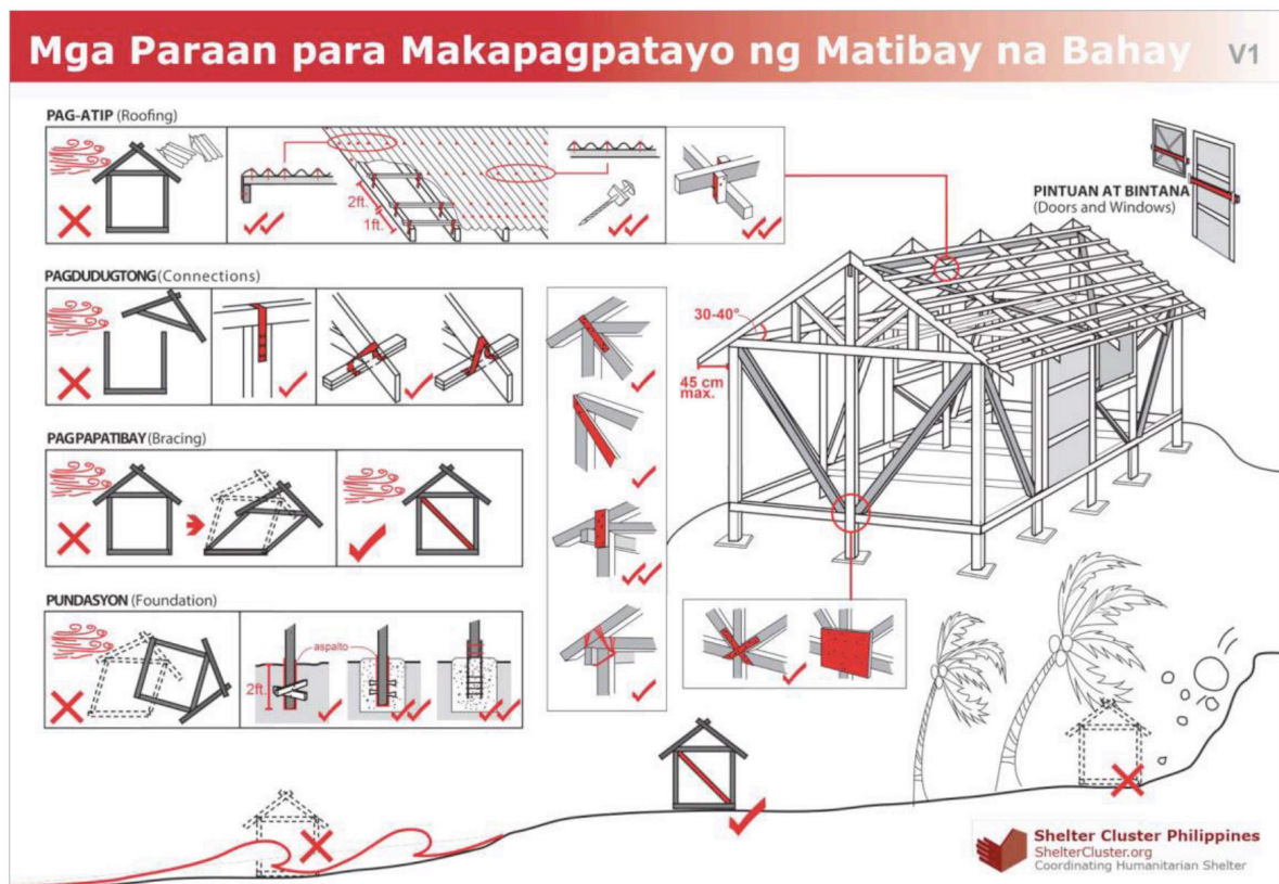
Figure 3. Joints for self-built houses in the Philippines (Shelter Cluster Philippines 2014a).
