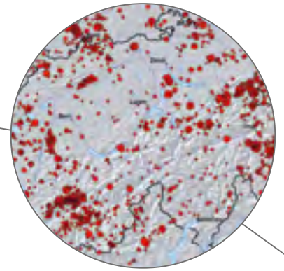
Earthquakes in Switzerland between 1975 and 2012.
