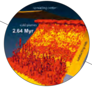
Cold upwelling plumes above a subducting plate.
