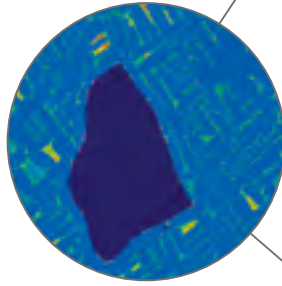
Inclusions of sulfides in the Cape York iron meteorite. The dark color indicates the low nickel concentration in the sulfide (approx. 3 cm long) compared to the surrounding metal, light blue / green in color.
