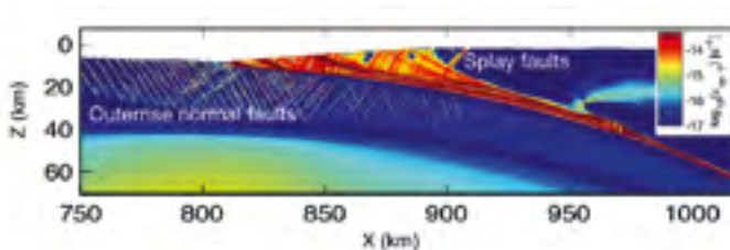
Numerical model of a subduction zone along which (approaching from the left) a tectonic plate submerges beneath a continent (right). Red-shaded regions represent fault zones that are responsible for a high rate of volcanic activity.
