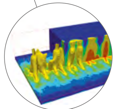
Numerical simulation of hot fluid ascending through fractured rock at mid-ocean ridges (1×3×4 km sized model). The hot fluids vent as “black smokers” but can also form large mineral deposits just below the ocean floor. Such simulation considerably helps to understand the complex thermodynamic and mechanical feedbacks occurring during fluid flow.
