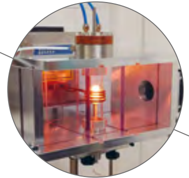
Custom-built furnace for simulating the early stages of planet formation under vacuum conditions.
