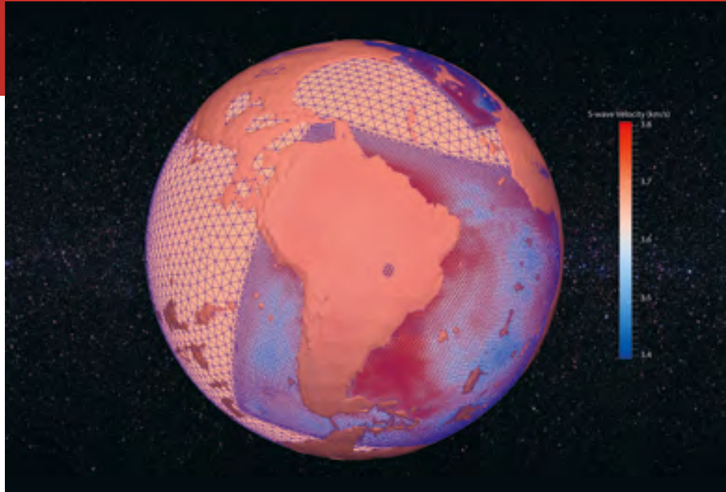
Model of the earth made up of millions of small tetrahedra, with topography (raised) and shear-wave velocity at 100 km depth.
