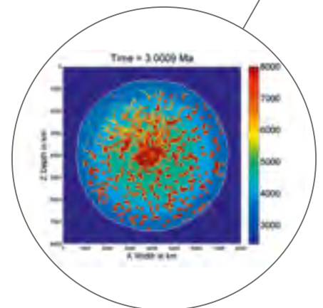
Computer simulation of the formation of Earth's core through the sinking of iron diapirs.
