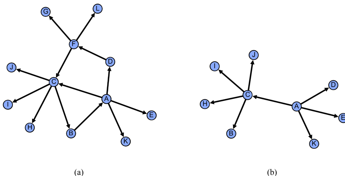
Figure 1. (a) An example of Twitter social graph created using the Follower relationship. Each node represents a Twitter user. An edge or arrow from node A to C, for example, shows that user C is following user A on Twitter. (b) A graph sampled from that in (a) using snowball sampling with starter nodes A and C.
