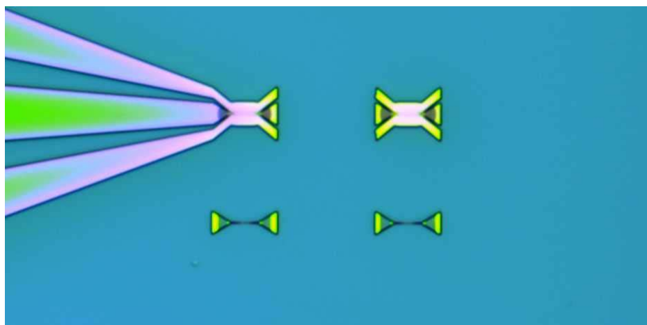
Microscopic image of a chip. Top left: functional modulator with electrical contacts; right: test modulator without electrical contact; below: test components. (Photograph: ETH Zurich)
