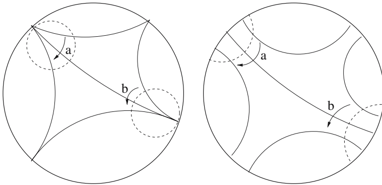
Fig. 1 \Gamma = \langle a, b \rangle and \Lambda = \langle a', b' \rangle
