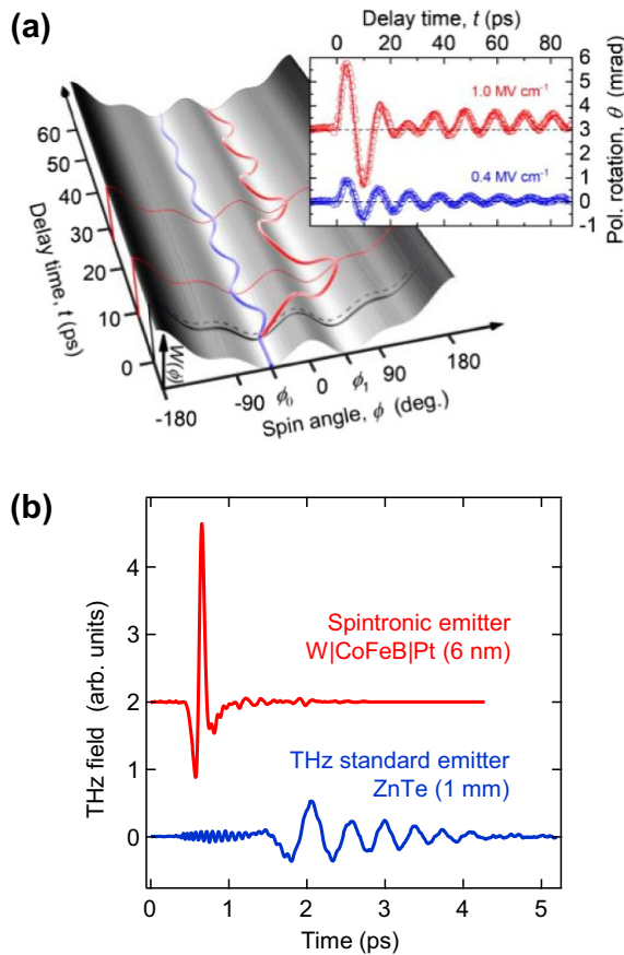
Figure 23. Applications of (a) THz spin torque and (b) THz spin transport. (a) Ballistic switching of antiferromagnetic order of TmFeO 3 . Simulations show that a THz field (peak 1 \text{ MV cm}^{-1} ) drives the antiferromagnetic order parameter from the minimum \Phi_0 of the potential W(\Phi) to the adjacent minimum \Phi_1 (red trajectory). A peak field of 0.4 \text{ MV cm}^{-1} is too small to induce switching (blue trajectory). In the measured magnetooptic probe signals \theta (see inset), the offset of the red curve for t > 40 \text{ ps} is an indicator that switching has occurred [160]. (b) Spintronic THz emitter. The red curve shows the THz signal obtained from an optimized spintronic trilayer, based on the principle of figure 22(c). The waveform is significantly larger and shorter and thus more broadband than that from a ZnTe standard emitter (blue curve) [161]. (a) Adapted by permission from Springer Nature Customer Service Centre GmbH: Nature [160] (2019). (b) Adapted by permission from Springer Nature Customer Service Centre GmbH: Nature Photonics [161] (2016).
