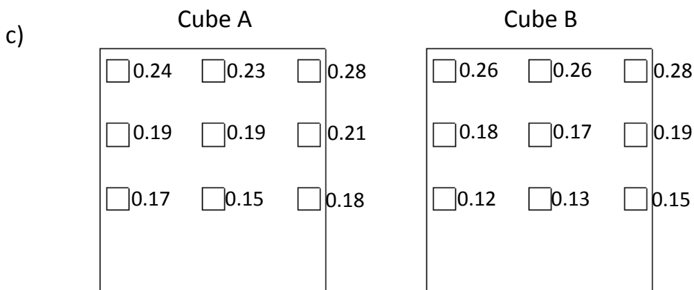
a) 10-minute meteorological data for the rain event. Wind speed is taken at 2.4 m height. b) Cumulative WDR amount measured by WDR gauges during the rain event and c) the catch ratio values at the end of the rain event on cube A and B.
