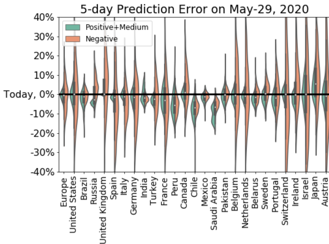
Figure 2. Five-day prediction error of the forecast performed 5 days ago for the total number of confirmed cases for the various countries/regions. The horizontal line corresponds to today’s empirical data. We show the full distribution of errors for each of the two scenarios..
