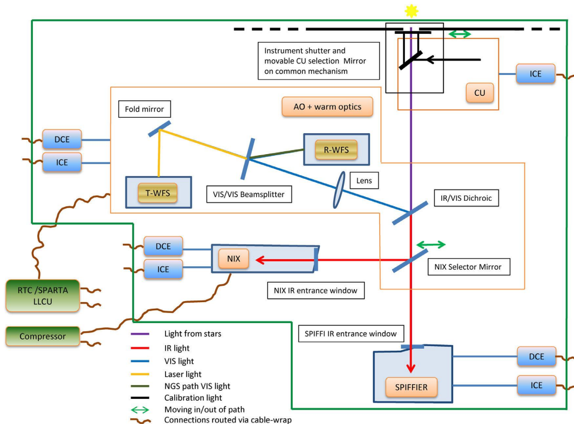
Figure 5. Sketch showing the concept for the optics in the central structure: how the light from the calibration unit is focused when the instrument shutter is closed; that the optical path goes directly to SPIFFIER passing only the IR/VIS dichroic which splits light off to the wavefront sensors; how a fold mirror can be moved in to reflect the light instead to NIX. Electronics connections are also shown.
