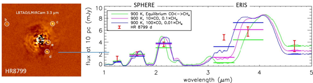
Figure 4. Illustration, using HR8799 d as an example, of how ERIS can contribute to resolving questions about atmosphere chemistry in exoplanets. 19 Left: L-band image of the HR8799 system indicating the four known planets. Right: JHK photometry from SPHERE cannot always distinguish equilibrium and non-equilibrium models, while possible LM measurements from ERIS may provide more decisive diagnostic power.
