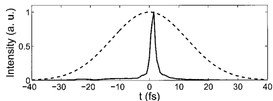
Fig. 4. Normalized intensity of the single-cycle pulse at z=115 cm. The dashed curve indicates the input pulse duration. The pulse has been averaged over a radius of 100 \mu\text{m} .
