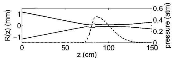
Fig. 1. Pressure distribution (dotted curve, scale on the right-hand axis) and computed beam width (continuous curve, scale at the left) along the propagation axis. The linear focus is at z=80 cm.
