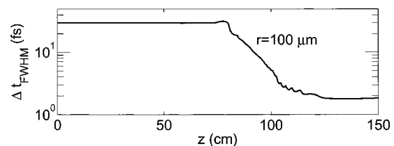
Fig. 3. Evolution of the pulse duration (FWHM) as a function of the propagation distance. The duration is computed after radial integration of the beam intensity over a beam radius of 100 \mu\text{m} .
