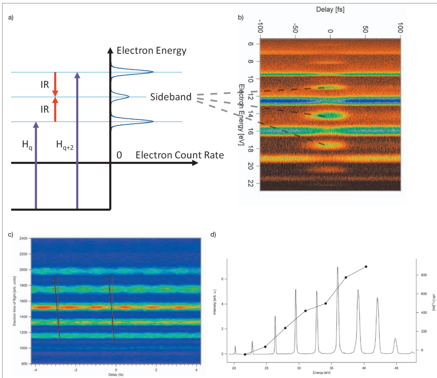
Fig. 2. Characterization of an attosecond pulse train (APT) [19,20] with the RABBITT technique [27] which determines the phase difference between two adjacent harmonics (top left). For the electron time-of-flight detection (top right) delay steps of 107 as ( i.e. 15 nm steps controlled with a piezo) with an acquisition time per step of 60 s have been applied. For a full RABBITT trace (bottom left) stable conditions for more than 30 hours are required. The recorded phase difference (bottom right) then determines the attochirp of the APT. Here we measured 450 as for the average pulse duration of the attosecond pulses within the APT with a transform limit of 160 as. With an additional 500-nm thick Al filter for dispersion compensation close to transform limited pulses can be achieved. [28]
