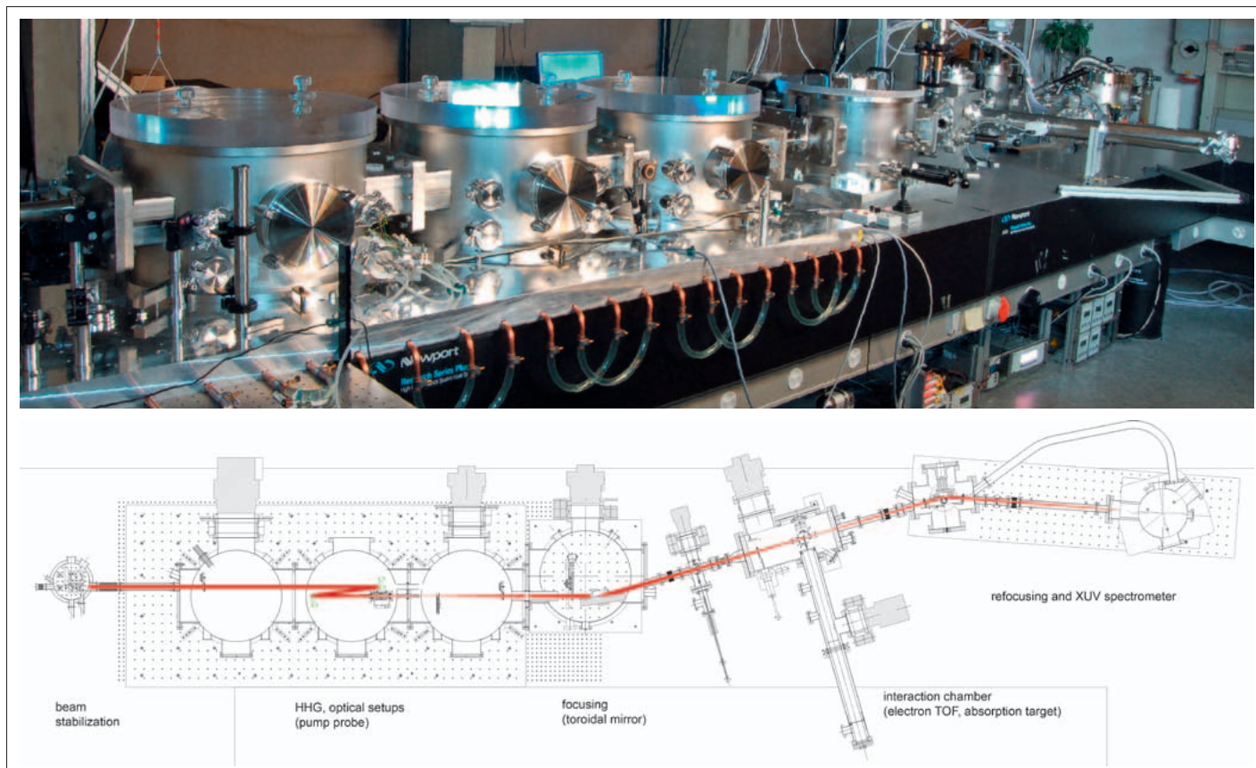
Fig. 1. Attoline at ETH Zurich. [19,20] From left to right: The first three identical chambers accommodate the high-harmonics generation target and an interferometer for pump-probe-like experiments. The next chamber contains a toroidal focusing mirror directing the VUV-XUV and infrared beams into the experimental target chamber. This chamber is equipped with a time-of-flight (TOF) spectrometer. On the most right-hand side, an XUV spectrometer is attached for photon diagnostics. Note that the high power infrared laser amplifier system is not shown here and comes from the left into the first chamber for HHG.
