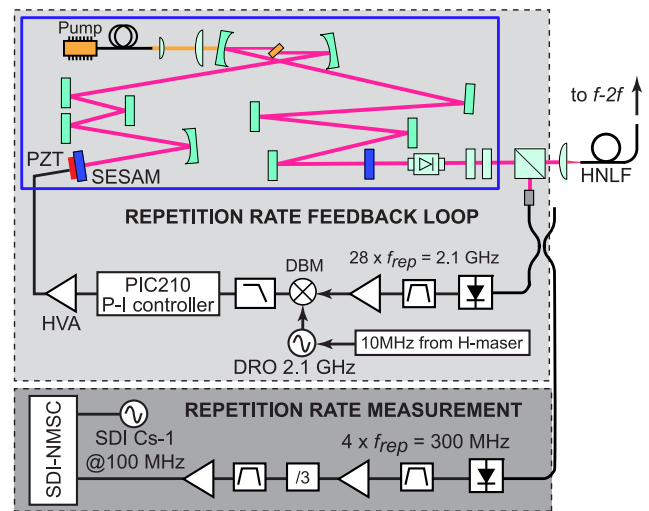
Fig. 5 Scheme of the repetition rate phase-lock loop (upper frame), including a 2.1-GHz DRO referenced to an H-maser, an analog phase comparator (double balanced mixer, DBM), a PI servo-controller, a high voltage amplifier (HVA) and feedback to the PZT to stabilize the laser cavity length. The lower frame shows the measurement scheme used to characterize the phase noise of the comb repetition rate against a low-noise 100-MHz synthesizer (SDI Cs-1) using a phase noise measurement system (SDI-NMSC)
