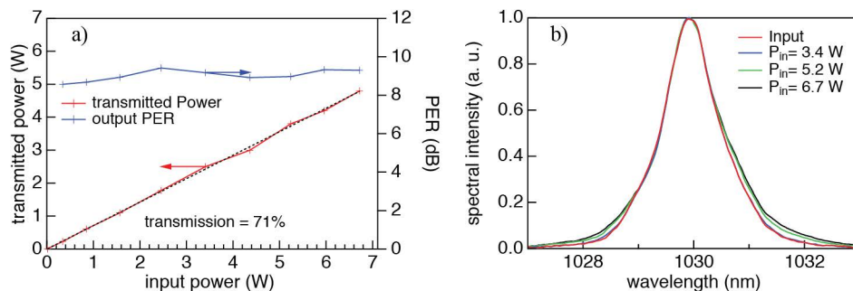
Fig. 4. Transmission properties of Kagome Type HC-PCF in air: (a) Transmission and corresponding PER for different input average powers (b) Output spectrum of the system through a Polarizing Beam Splitter (PBS) for different input average powers.
