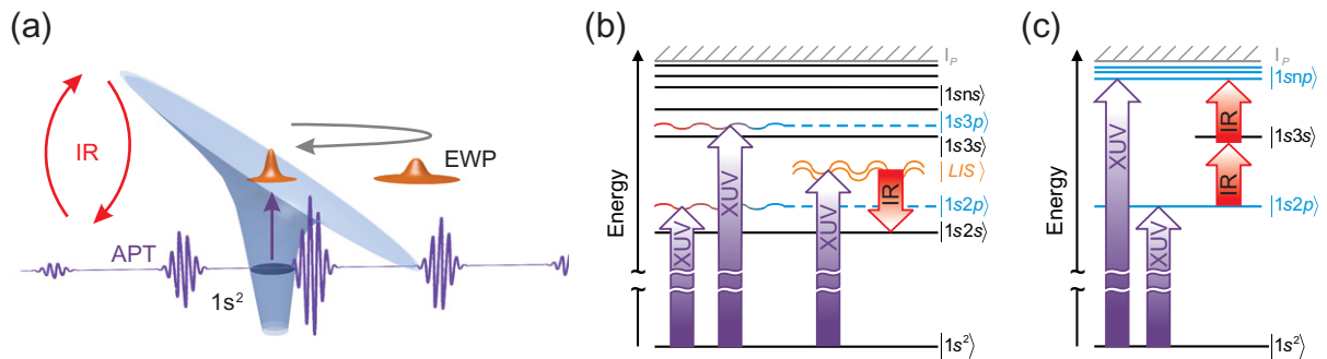
Figure 1. Schematic of the main mechanisms proposed to explain the oscillation of the photoabsorption probability in the case of APT (a) and SAP excitation (b)–(c). (a) Interference between two parts of a transiently bound EWP excited by subsequent pulses in the APT [2, 5]. (b) Resonant absorption lines of the 1np series affected by sub-cycle ac Stark shift and light-induced structures associated with two-photon/two-color processes [6, 7]. IR dressed states are represented with wavy lines. (c) ‘Which way’ interference between direct extreme-ultraviolet (XUV) excitation and an IR-assisted two-color transition [8–10].
