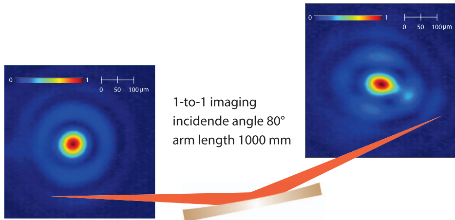
FIG. 9. Beam profile in the 1st (left) and 2nd (right) focus for the delayed beam. For the collinear recombination of XUV and IR beam, the central part of the IR beam is cut out by the DM in Fig. 2 and the beam is clipped by an iris to reduce the intensity. This explains the weak interference rings. As the XUV pulse only overlaps with the central part of the pulse, these pedestals in the transverse beam profile are not important.
