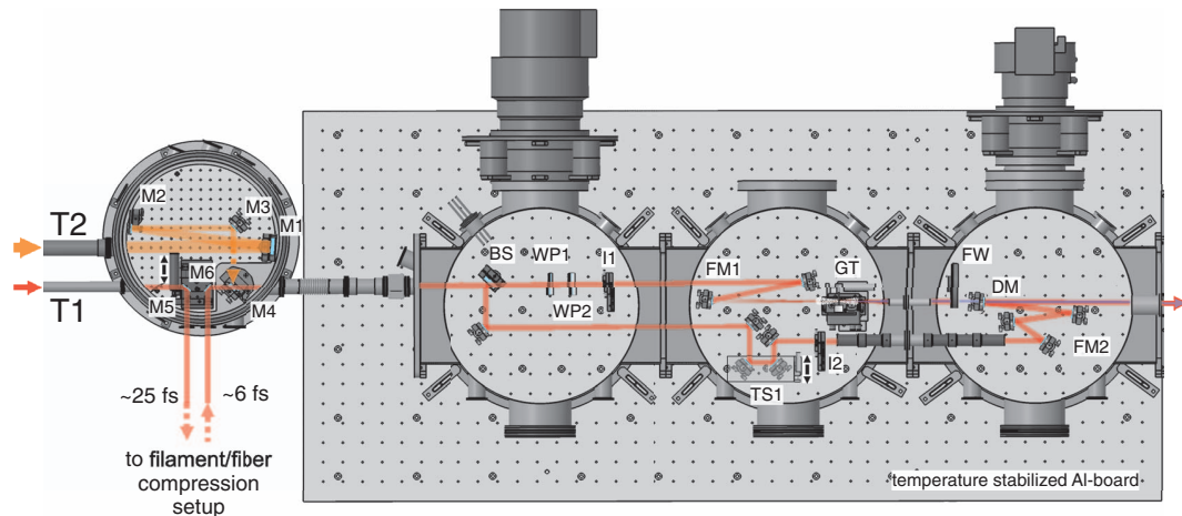
FIG. 2. Coupling and generation chambers: In the first chamber the two outputs from the laser system are coupled into the attolite. The three adjacent identical chambers form the pump-probe interferometer. The IR beam is split into two parts by a beam splitter (BS) located in the first chamber. The more intense part passes the beam splitter and is focused into the gas target (GT) to generate high-order harmonics. The weaker part is delayed and subsequently recombined with the XUV beam with a drilled mirror (DM) which contains a small center hole for the XUV beam and still reflects most of the larger IR beam. For improved stability the entire interferometer is placed onto a temperature-stabilized aluminum board on top of a standard commercial laser table.
