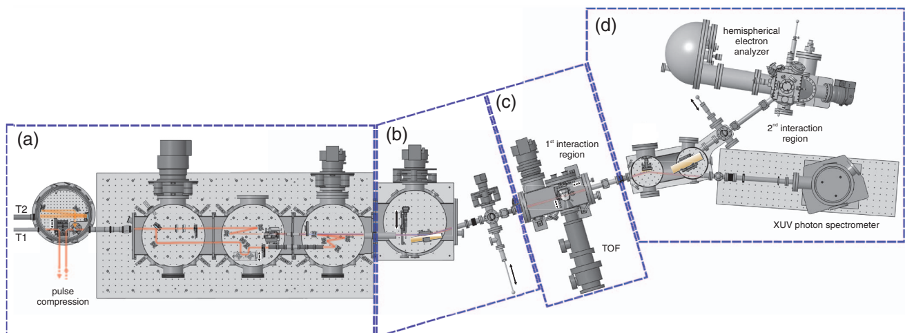
FIG. 1. Experimental setup consisting of four main blocks (delimited by the dashed frames: (a) laser beam coupling and XUV generation chambers, (b) diagnostics and focusing chamber, (c) first interaction chamber with a time-of-flight (TOF) spectrometer, and (d) second refocusing and interaction chambers together with the photon spectrometer. The hemispherical electron analyzer placed in the second interaction region is not a permanent component of the attoline, but represents an example for an exchangeable end station (see Sec. III B).
