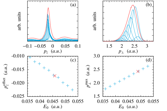
FIG. 7. Focal volume averaging and the measured effective intensity: (a) for the ridge in the transverse PMD in linearly polarized laser field; (b) for the PMD radius in the polarization plane in a circularly polarized laser field. The distributions at each laser intensity are shown in blue. The position of the maxima in (a) and (b) are shown in (c) and (d), respectively. The focal averaged intensity deduced from the ridge in the case of linear polarization [red cross in (c)] is different from that deduced from the case of a circular polarization [red cross in (d)].
