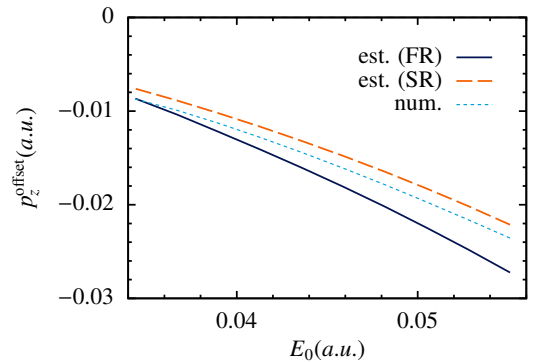
FIG. 6. Nondipole shift of the PMD ridge at p_x = 0.5 a.u. vs the laser field strength: The analytical prediction of Eq. (14), with \phi_r corresponding to the first, fast recollision (FR) (solid), and corresponding to the second, slow recollision (SR) (long-dashed); The numerically found classical trajectory that end at the ridge (short-dashed).
