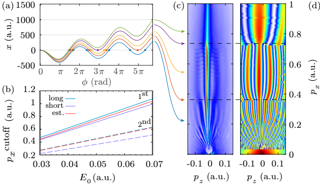
FIG. 3. (a) Schematic examples of recolliding trajectories: the trajectory with a single recollision (recollisions are indicated by dots) exists for 0.2E_0/\omega < |p_x| < E_0/\omega (green); the second and third returns exist for trajectories up to 0.1E_0/\omega < |p_x| < 0.2E_0/\omega (yellow), four or more recollisions exist at |p_x| < 0.1E_0/\omega (blue), and so on, see Eqs. (8)-(9). The momentum transfer at a recollision is enhanced for the specific trajectories (purple and red) when the recollision velocity is vanishing (slow recollision) [74, 75]. (b) The smallest p_x cutoff for trajectories with a single recollision (solid), corresponding to the 1st slow recollision, and three recollisions (dashed), corresponding to the 2nd slow recollision; (long) The slow recollision condition in a monochromatic laser field; (short) The slow recollision conditions in a 50 fs laser pulse, and (est.) The analytical estimates of Eqs. (8) and (9). The cutoffs are clearly visible in the PMDs from the QTMC (c) and simplified model simulations (d). For the simulations the laser and atom parameters are the same as in Fig. 1.
