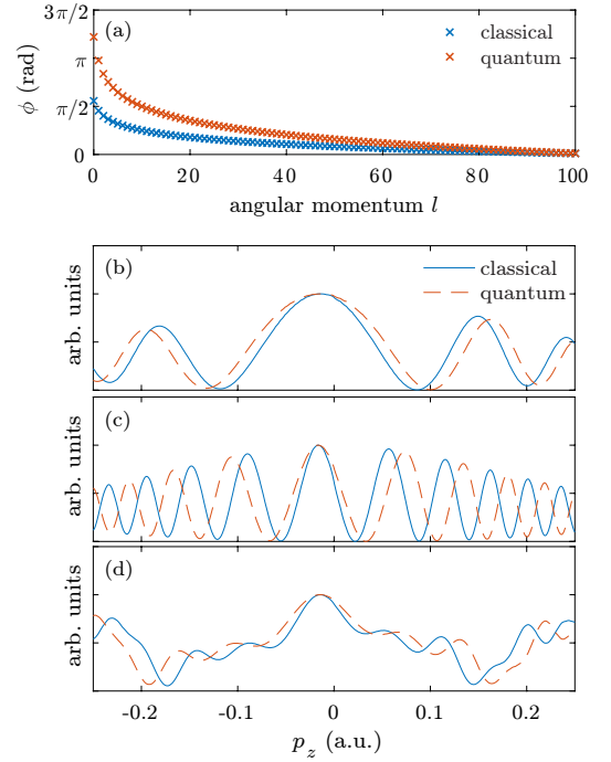
FIG. 8. Comparison of quantum and quasiclassical rescollision phases (a). The lineouts of the 2D calculation of PMD at p_x = 0.9 a.u. on panel (b) and p_x = 0.5 a.u. on panels (c) and (d) taking into account two (b) and (c) or all eight (d) interfering trajectories. The blue full lines represent the 2D calculation with the common classical SFA Coulomb phase and the red dashed lines the results corrected by the quantum phase at each rescattering.
