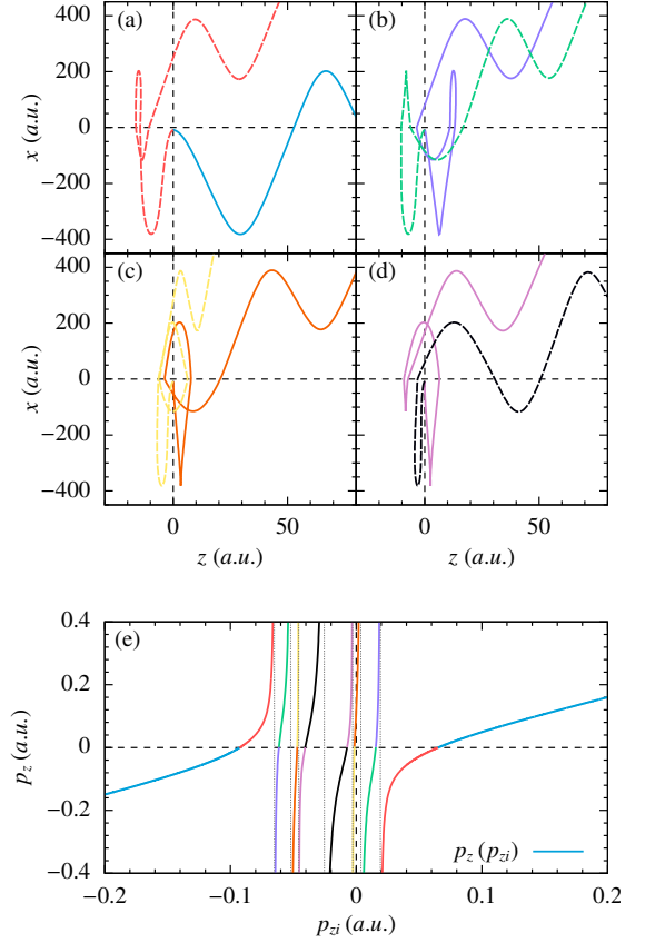
FIG. 4. The examples of 8 types of trajectories identified in the QTMC simulation at p_x = 0.5 : (a) Trajectories with no significant rescattering (blue), and with a significant rescattering at the 3rd recollision (red), (b) Trajectories with a significant rescattering at the 2nd recollision (green), and at the 2nd or 3rd recollisions (violet), (c) at all recollisions (yellow), or at the 1st and 2nd recollisions (coral), (d) at the 1st (black), or at 1st and 3rd recollisions (magenta). (e) The final transverse momentum, p_z vs the initial, p_{zi} , which determined the type of trajectories indicated by color. The color of trajectories in panels (a)-(d) indicate the type according to the panel (e). The type of pair trajectories in each of panels (a)-(d) is interchanged with continuous variation of p_{zi} (e.g. blue-type of trajectory becomes red-type at decreasing p_{zi} , at p_{zi} > 0 ).
