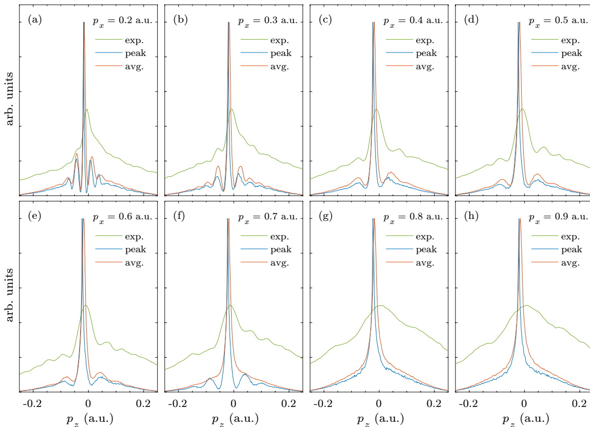
FIG. 9. Comparison of the lineouts obtained from experiment (exp.) and QTMC calculation with a focal averaged intensity (avg.) and the peak intensity (peak) for different positions along the laser polarization axis p_x .
