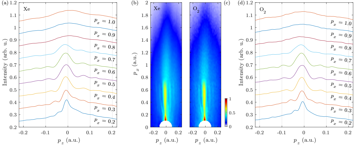
FIG. 2. Lineouts of the experimental PMDs from strong-field ionization at linear polarization of the two targets xenon and oxygen at different p_x positions along the laser polarization axis (in atomic units). The integration band for the lineouts in p_x direction has a width of 0.04 a.u.. The lineouts are normalized to the integrated signal and for clarity of the figure offset in absolute intensity by the value of the p_x position. Both targets show a very similar holography pattern with cutoffs for the number of interference maxima around p_x = 0.35 a.u. and p_x = 0.75 a.u. and an asymmetry in the intensity of the corresponding left and right sidelobe peak in laser beam propagation direction p_z (for details see text).
