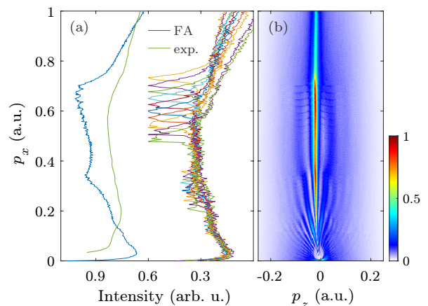
FIG. 5. (a) Longitudinal momentum distribution. The distributions for 10 sampling intensities are shown as overlapping multicolor lines. The peaks for each intensity correspond to the 1 th transition points (cutoff momenta) of the holography pattern for the given intensity. The distribution of the total focal averaged spectrum from (b) can be found in (a) as blue line and the distribution from the experimental data as green line. The knee position of the p_x -distribution at p_x \approx 0.75 a.u. corresponds to the transition border of the topological structures for the intensity very close to the peak intensity.
