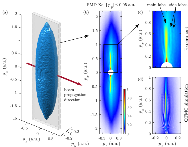
FIG. 1. Experimental PMD from strong-field ionization of xenon atoms: (a) Tomographic reconstruction of the 3D PMD, (b) measured PMD slice within |p_y| \leq 0.05 a.u., (c) PMD enlarged in, with removal of the zero energy spot due to electrons captured in Rydberg states. A 6-cycle laser pulse of linear polarization is used with an intensity of 5.8 \times 10^{13} W cm ^{-2} , and a wavelength of 3.4 \mu m, (d) corresponding semiclassical simulation.
