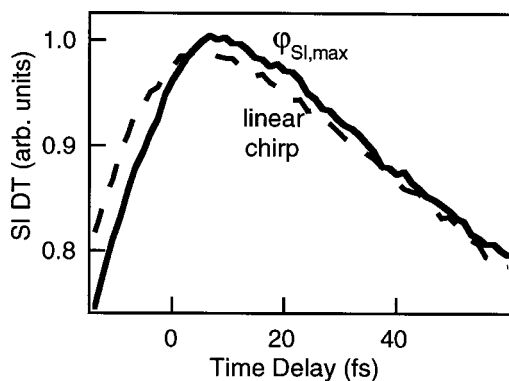
Fig. 7. SI DT for the optimized phase \varphi_{\text{SI,max}} and for the optimization of only the slope of a linear chirp. Temperature is 300 K; N_{\text{exc}} \approx 3 \times 10^{17} \text{ cm}^{-3} .
