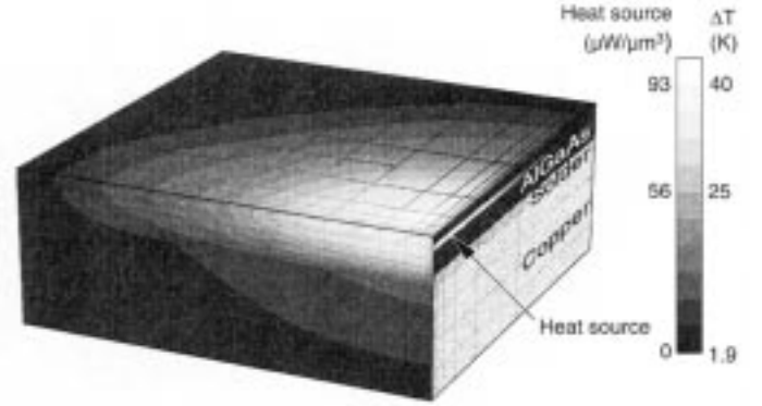
Fig. 5. Temperature distribution. The gain structure is soldered on a copper heat sink. The active area is heated with 512 mW on a pump spot with a 56.6- \mu\text{m} radius. Only the close surrounding of the heat source is shown, while the simulation expands much further.
