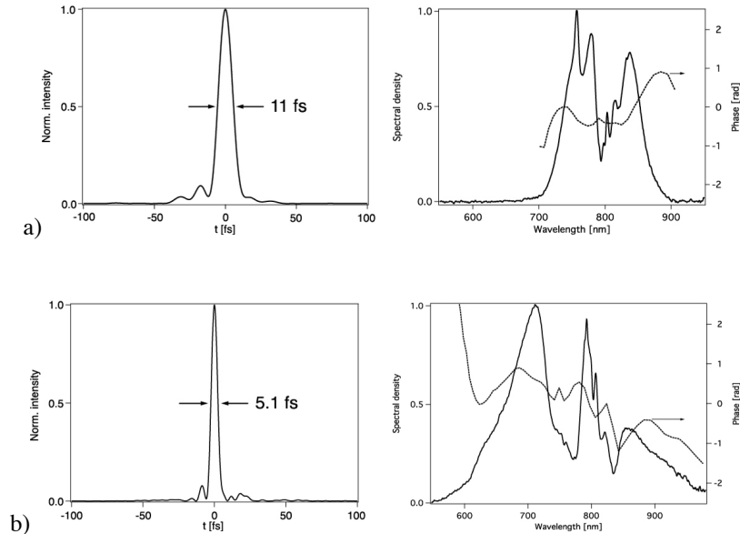
Fig. 6. Pulse and associated spectrum and phase a) after the first filament cell (11 fs) b) after the second filament cell (5.1 fs)
