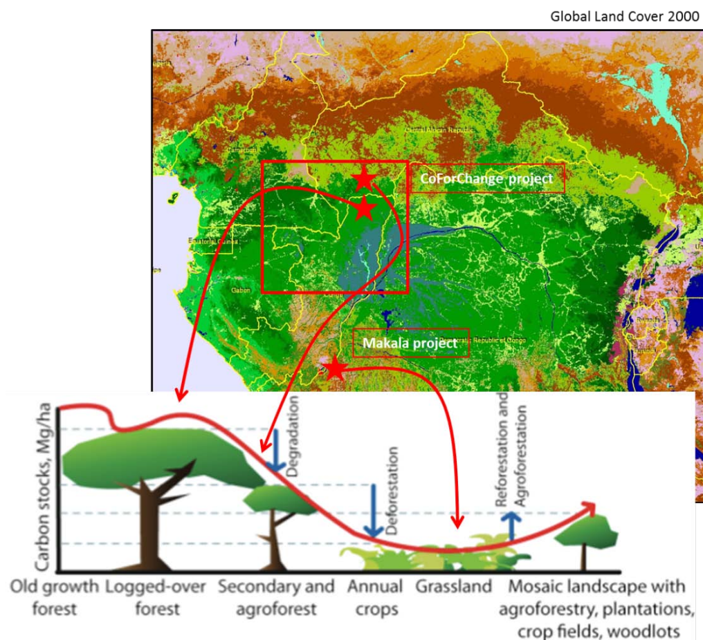
Figure 1: Location of the study sites and situation on the forest transition curve (source: http://www.cifor.org/crp6/research-portfolio.html )
